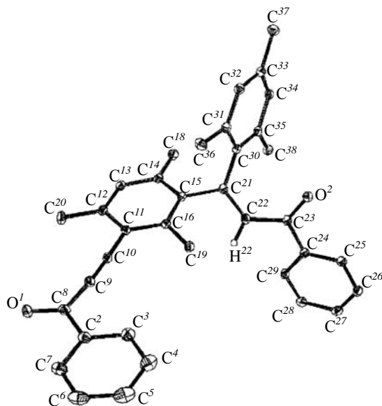
Fig. 1. Molecular structure of (E) -3-(2,4,6-trimethylphenyl)-3-[2,4,6-trimethyl-3-(phenylcarbonyl)ethynyl]phenyl]-1-phenylpropanone E -( VIIb ).
